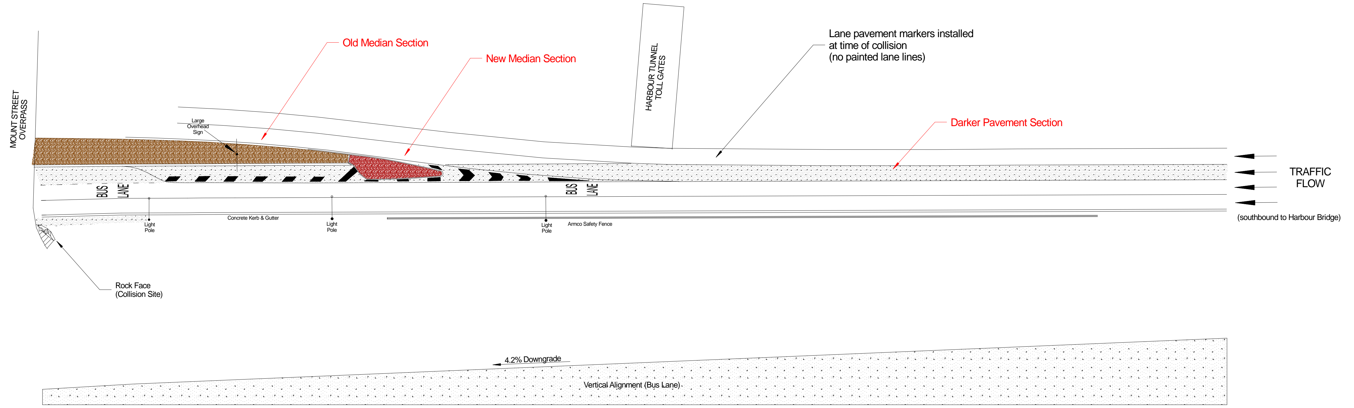
Longitudinal Section - Warringah Expressway Hor Scale 1:400 Ver Scale 1:400
